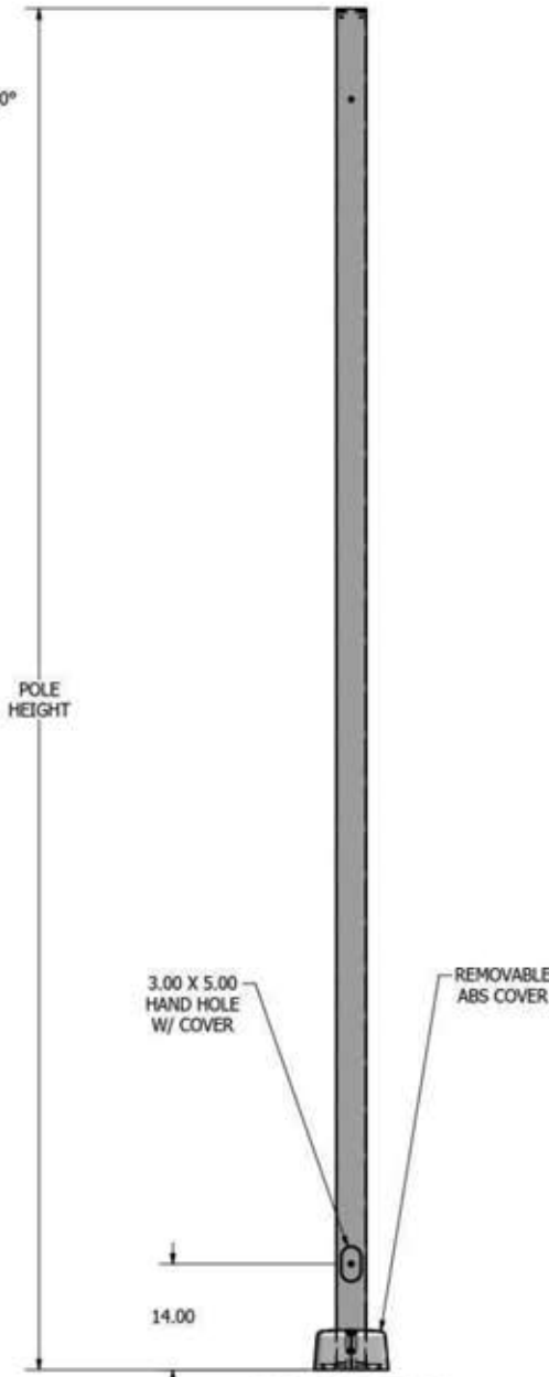
POLE DETAIL
