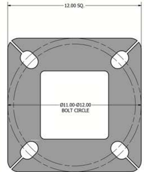
12.00 X 12.00 X 1.00 THK. BASE PLATE
