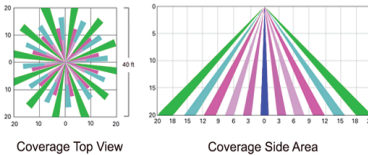
10' - 40' Mounting Height
