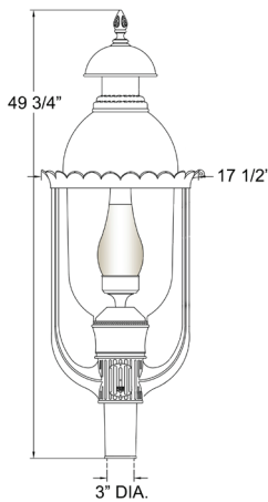
H1630CH Style H: 49 3/4" W: 17 1/2" EPA: 2.60 Fitter: 3" Diameter
