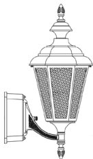
H9962RLED H: 33 1/8" W: 13 3/4" Proj: 18" T/O: 24 1/4"
